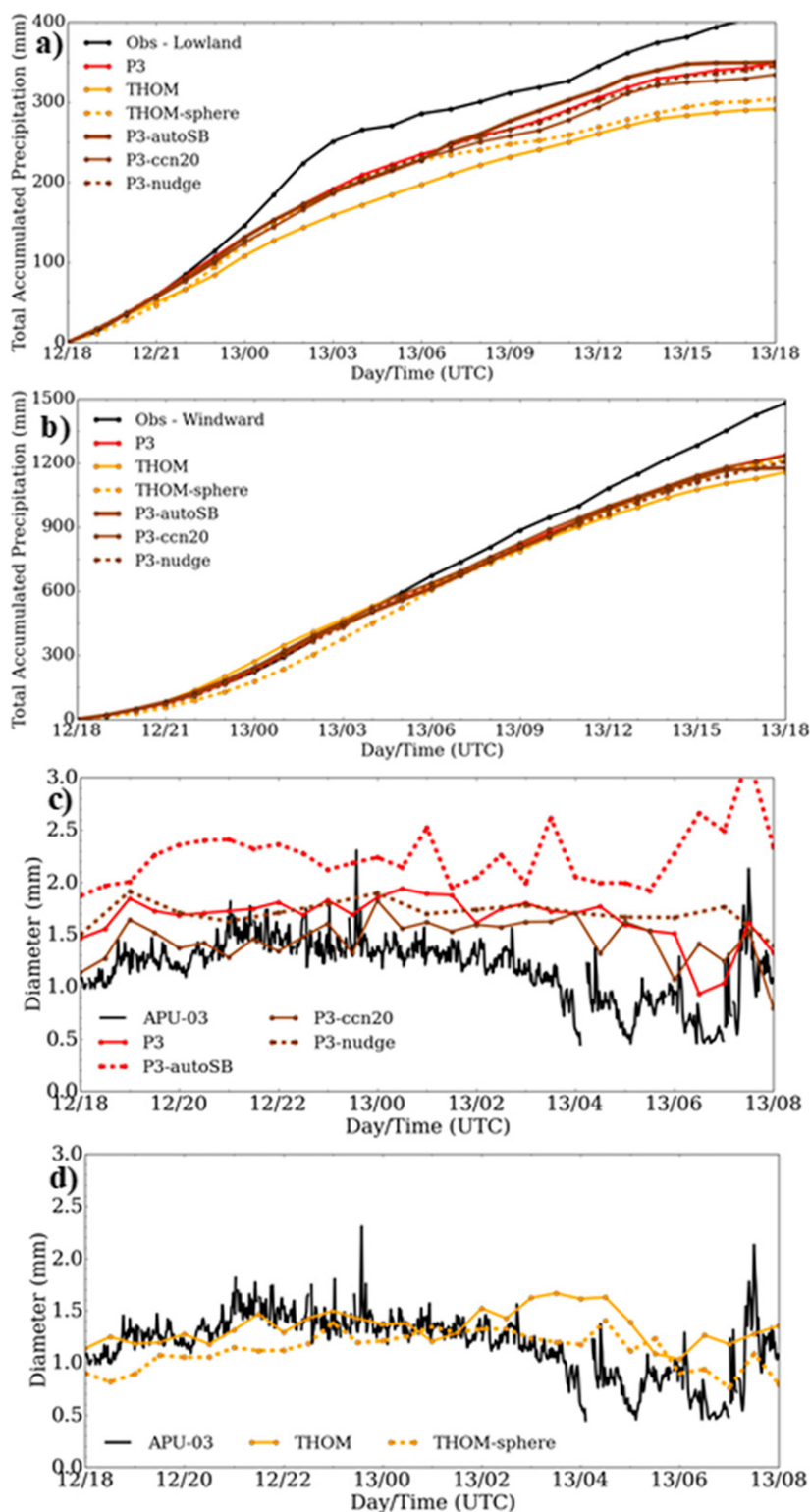
FIG. 16. (a) Lowland and (b) windward observed precipitation time series constructed from site locations denoted in white and blue, respectively, in Fig. 1a. Model precipitation time series constructed using bilinear interpolation of 4 nearest model grid points to site location for P3, THOM, THOM-sphere, P3-autoSB, P3-ccn20, and P3-nudge runs. (c) Mass-weighted mean rain diameters ( D_m ) from the APU disdrometer at Fishery
