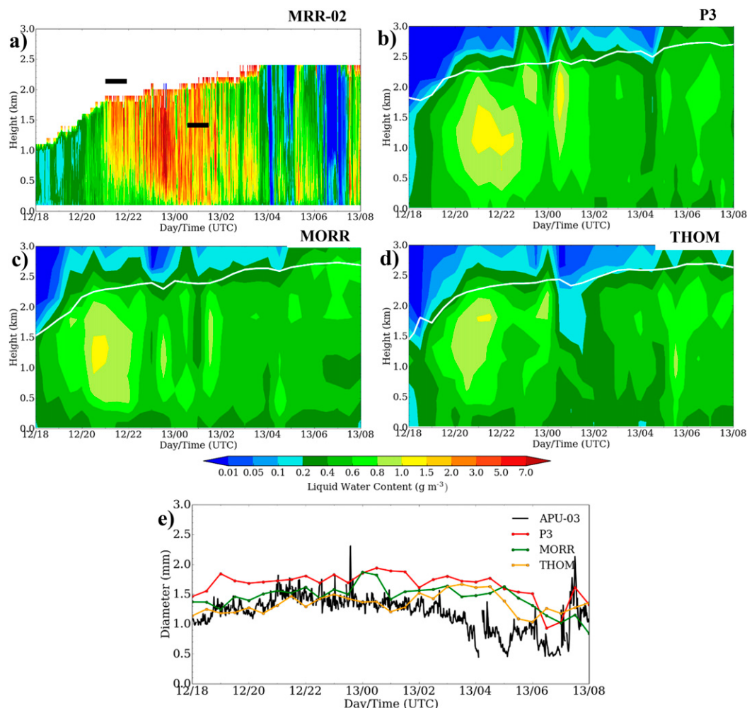
FIG. 11. (a) MRR LWC from 1800 UTC 12 Nov to 0800 UTC 13 Nov at Fishery site (MRR-02). Data unavailable after 0800 UTC 13 Nov due to power outage. Approximate base height of turbulent layer estimated from NPOL EDR is shown by horizontal black bars. Simulated LWC at Fishery site for (b) P3, (c) MORR, and (d) THOM schemes. Freezing level (273.15 K) denoted by white line. (e) D_m from the APU disdrometer at Fishery (APU-03) for same time period as MRR vs simulated rain diameters within the BMPs. Bilinear interpolation of 4 nearest model grid points used to calculate LWC and rain diameters from BMPs at Fishery site.
