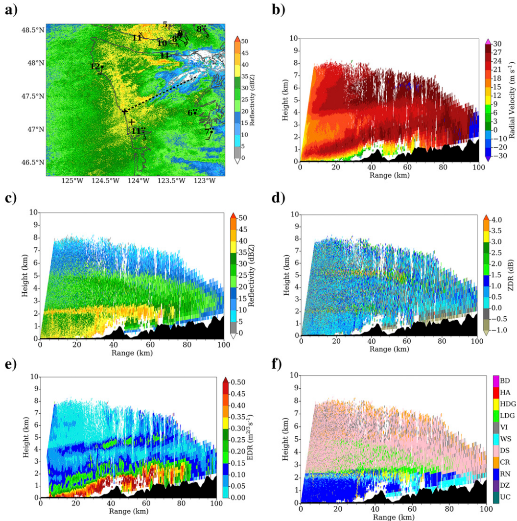
FIG. 9. As in Fig. 6, but (a) at approximately 0030 UTC 13 Nov 2015 for NPOL/NEXRAD PPI scan and (b)–(f) 0116 UTC for NPOL RHI scan. (f) Refer to hydrometeor types listed in Fig. 6 caption.
