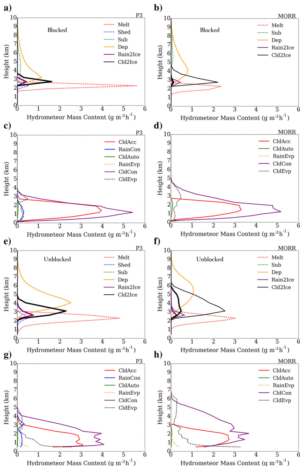
FIG. 15. Averaged vertical profiles of cold microphysical process rates ( \text{g m}^{-3} \text{h}^{-1} ) along 0–25 km section of NPOL 54° azimuthal scan for 2-h period (2030–2230 UTC 12 Nov) during stable blocked flow, rime layer period in (a) P3 and (b) MORR simulations. Cold processes include melting (“Melt”), shedding (“Shed”), sublimation (“Sub”), deposition (“Dep”), conversion of rain to ice (“Rain2Ice”), and conversion of cloud to ice (“Cld2Ice”). We sum the individual process rates associated with ice, snow, and graupel from
