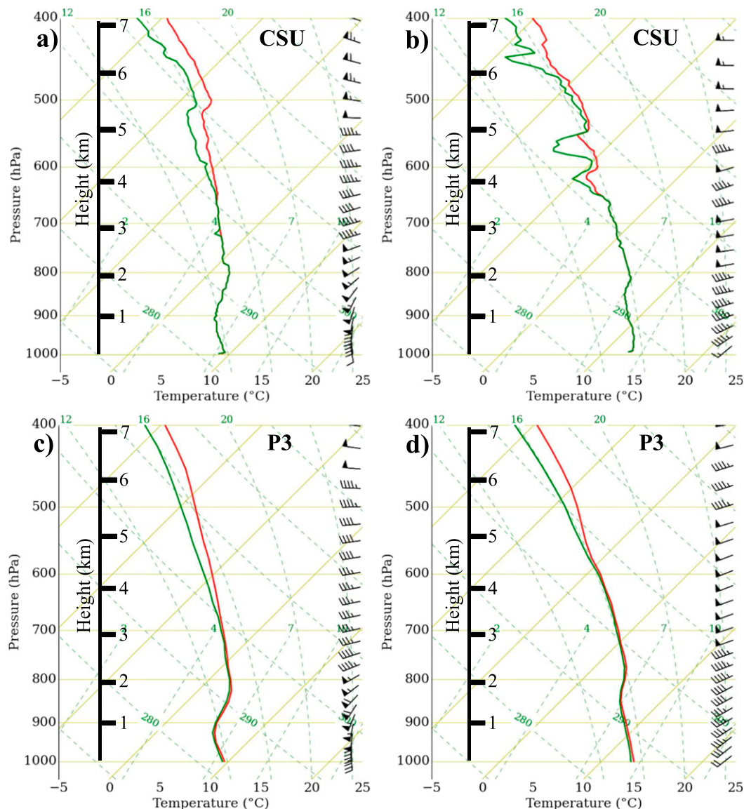
FIG. 3. CSU NPOL observed soundings at (a) 2100 UTC 12 Nov and (b) 0600 UTC 13 Nov. Model sounding from P3 simulation at (c) 2030 UTC 12 Nov and (d) 0530 UTC 13 Nov calculated by averaging the nearest 25 grid points to the NPOL site.
