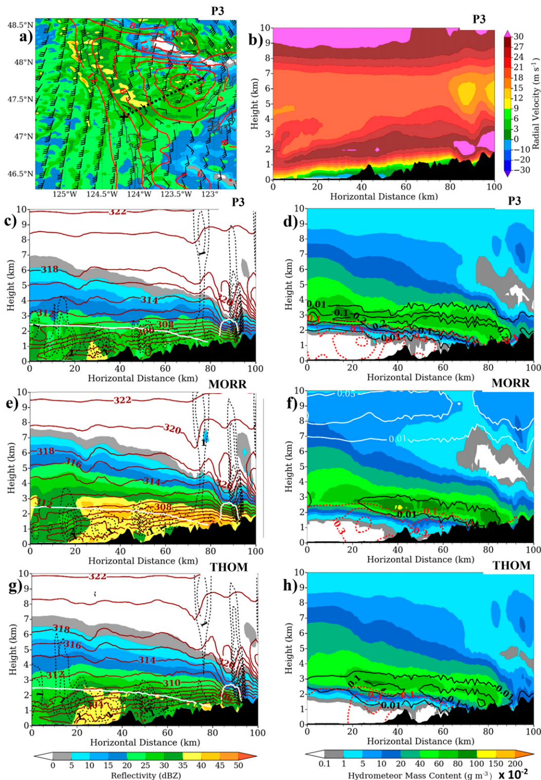
FIG. 7. (a) WRF P3 reflectivity (shaded) at 2100 UTC 12 Nov 2015 from the lowest model vertical level, along with the predicted 2-m temperature (red, contoured every 2^{\circ}\text{C} ) and 10-m wind speed (1 full barb = 10 kt). NPOL location indicated by black cross, with approximate path of NPOL 54^{\circ} RHI scan in dashed black. Cross sections along NPOL RHI 54^{\circ} azimuthal scan in Fig. 6. (b) Simulated P3 radial velocity and (c) reflectivity (shaded in dBZ), \theta_e^* (solid maroon, contoured every 2 K), and vertical velocity (dashed black, contoured every 0.5 \text{ m s}^{-1} ) at 2130 UTC 12 Nov. Solid white line represents the freezing level at 273 K. (d) Simulated P3 hydrometeor mass
