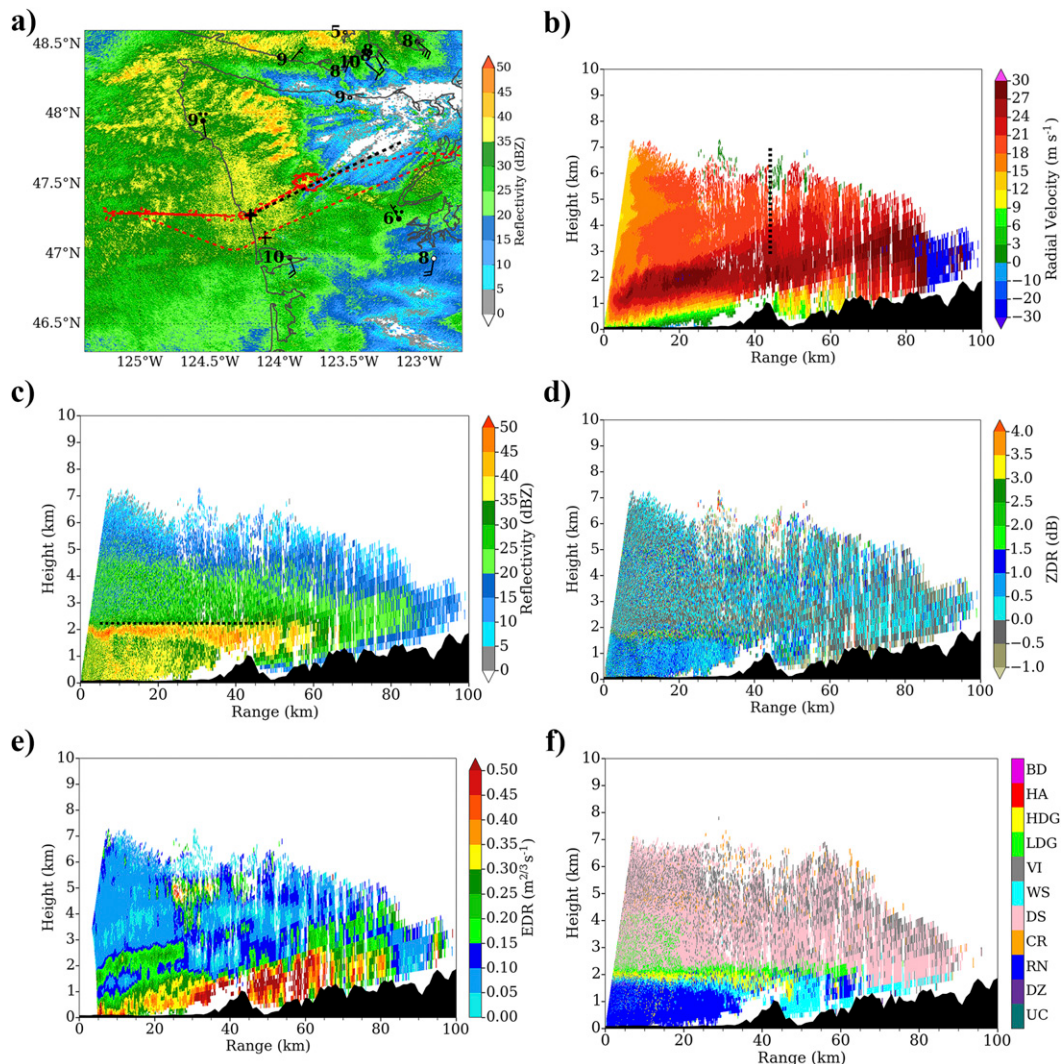
FIG. 6. (a) Radar reflectivity from the NPOL and NEXRAD (KATX, KLGX, KRTX) 0.5° elevation scans (shaded in dBZ) at approximately 2100 UTC 12 Nov 2015. The 2-m temperature (°C) and 10-m wind speed (1 full barb = 10 kt) at 2100 UTC from ASOS stations are also shown. Aircraft track highlighted in dashed red with the spiral indicated by circular patterns over windward slopes and NPOL RHI 54° azimuthal scan shown in dashed black. Radar variables from the NPOL RHI 54° scan at 2132 UTC 12 Nov 2015: (b) radial velocity (aliased at the 80–100 km range), (c) reflectivity, (d) ZDR, (e) EDR, and (f) hydrometeor classification. Location of aircraft spiral denoted by vertical dashed line in (b) and approximate location of 0°C level from CSU sounding shown by horizontal dashed line in (c). Hydrometeor classifications are defined as (from bottom to top) UC = unclassified, DZ = drizzle, RN = rain, CR = ice crystals, DS = dry snow, WS = wet snow, VI = vertical ice, LDG = low-density graupel, HDG = high-density graupel, HA = hail, and BD = big drops/melting hail.
