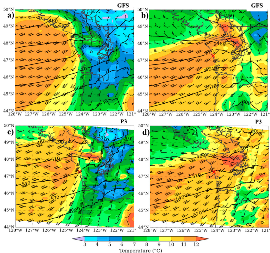
FIG. 2. GFS 950 hPa temperature (shaded), geopotential heights (solid black, contoured every 30 m), and winds [1 full barb = 10 kt (1 kt \approx 0.51 m s ^{-1} )] at (a) 0000 and (b) 1200 UTC 13 Nov 2015. (c),(d) As in (a),(b), but for P3 simulation results from the WRF 1-km grid.
