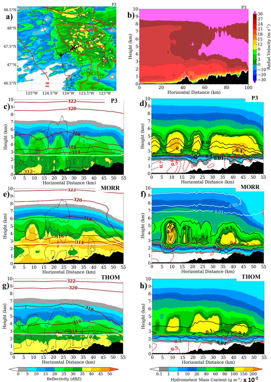
FIG. 13. As in Fig. 7, but at approximately 0730 UTC 13 Nov and along the DOW RHI 64° azimuthal scan. (a) DOW location denoted by black \times with corresponding 64° scan in dashed white.
