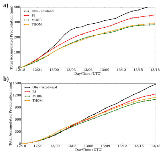
FIG. 4. (a) Lowland and (b) windward observed precipitation time series constructed from site locations denoted in white and blue, respectively, in Fig. 1a. Model precipitation time series constructed using bilinear interpolation of 4 nearest model grid points to site location for P3, MORR, and THOM schemes.
