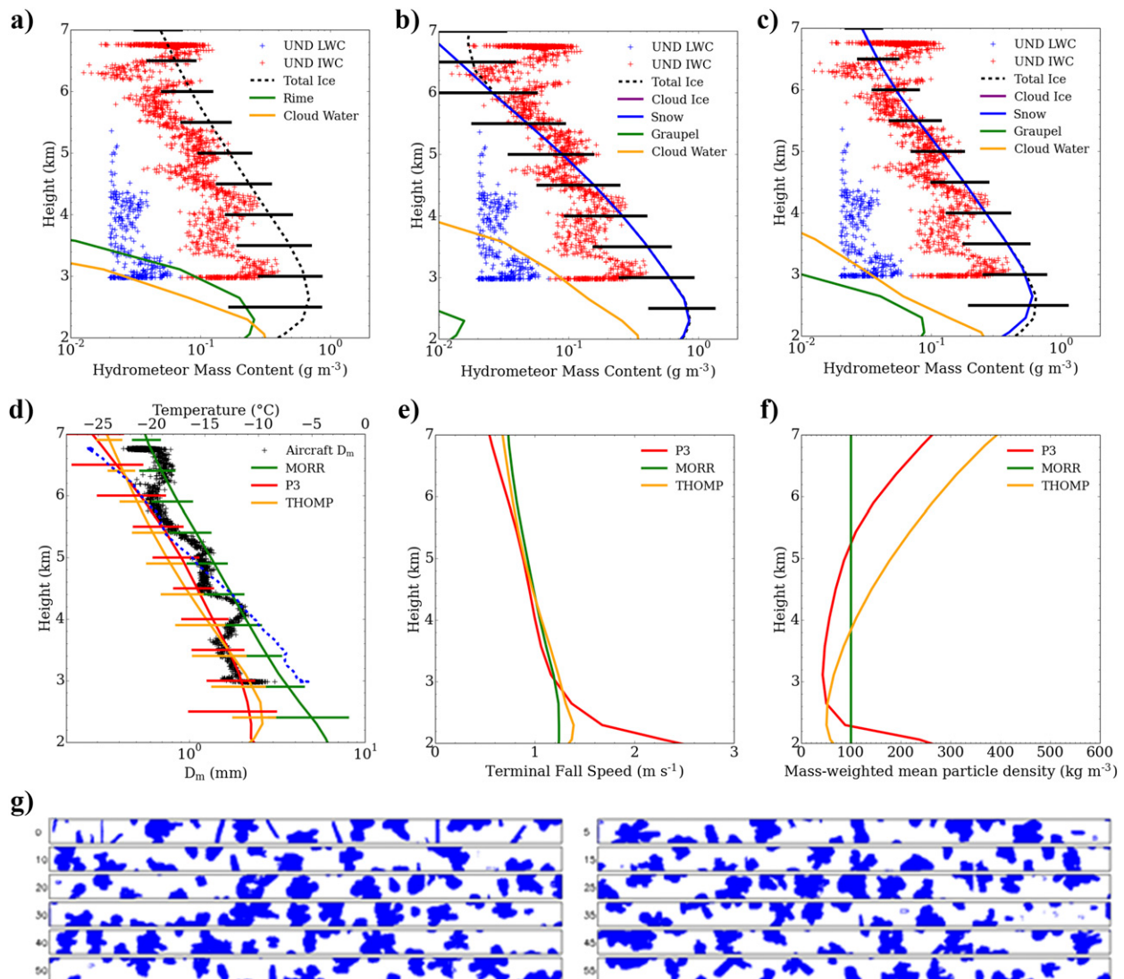
FIG. 8. Mean vertical profiles of hydrometeor content calculated from (a) P3, (b) MORR, and (c) THOM at 2000 UTC 12 Nov 2015 using the nearest 200 grid points to the location of the aircraft spiral. Horizontal bars represent the range of the simulated total ice mass content at 0.5 km altitude increments. King and Nevzorov probe measurements of cloud liquid water content (blue cross) and total ice content (red cross), respectively, during the ascending spiral between 1940 and 2010 UTC 12 Nov (Fig. 6a). (d) Mean vertical profiles of mass-weighted mean diameter ( D_m ) calculated from the HVPS measurements during the spiral vs D_m calculated from BMP output at same time and location as (a)–(c). Temperature profile measured by aircraft is shown in dashed blue. (e) Simulated mass-weighted terminal fall speed and (f) mass-weighted mean particle density for precipitating ice species ( \rho_{pi} ) within the schemes (no aircraft estimates available). (g) Particle imagery from 2D-C acquired in 5-s intervals (shown to left of each image) at 1943 UTC and approximately 3 km in height during aircraft spiral.
